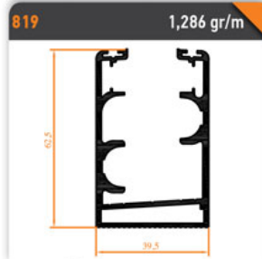
819 1,286 gr/m Düz Kasa Üstten Fitilli Profili Flat Body Mounted Profile
