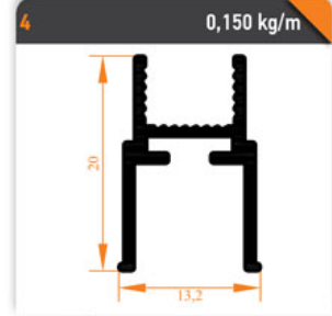
Orta H Fitil Middle H Seal
