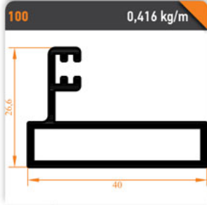
Dar Yan Dikme Thin Side Pillar
