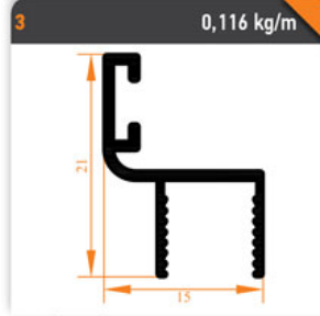
Küçük H Fitil Small H Seal
