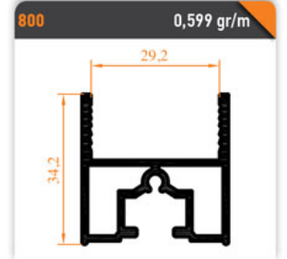
800 0,599 gr/m Isıcam Baza Double Glazing Base
