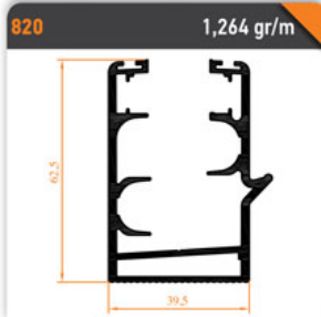
820 1,264 gr/m Oluklu Kasa Üstten Fitilli Profili Corrugated Case Top Heater Profile
