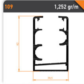
Düz Kasa Profil Corrugated Case Profile
