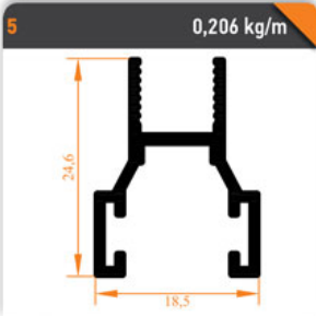
Büyük H Fitil Big H Seal
