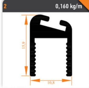
Küçük D Fitil Small D Seal
