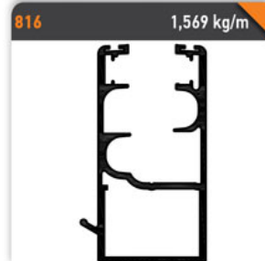
816 1,569 kg/m Fitilli Büyük Oluklu Kasa Large Corrugated Case
